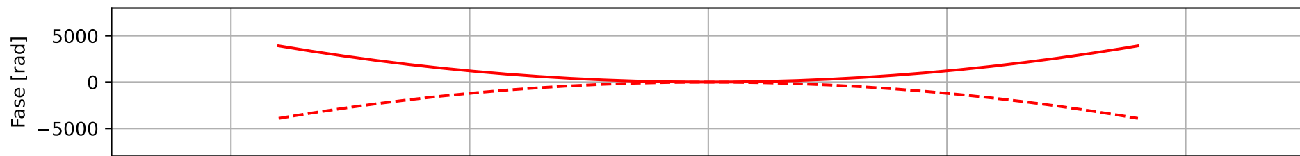
BR = 120 GBd
